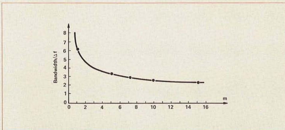
Figure 16. Bandwidth requirements vs. modulation index, m .
