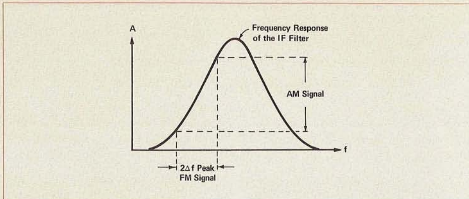
Figure 23. Slope detection of an FM signal.
