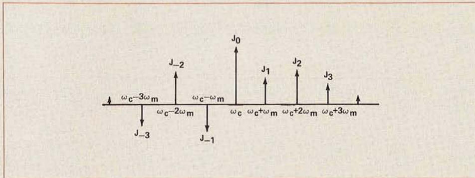
Figure I-5. Composition of an FM wave into sidebands.
