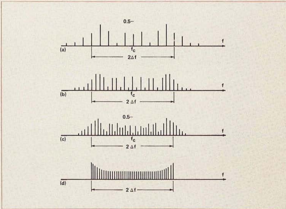
Figure 13. Amplitude-frequency spectrum, FM signal (amplitude of \Delta f fixed, f_m decreasing). (a) m = 5 ; (b) m = 10 ; (c) m = 15 ; (d) m \rightarrow \infty .
