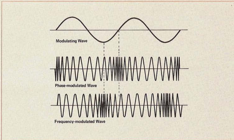
Figure 10. Phase and frequency modulation of a sine wave carrier by a sine wave signal.
