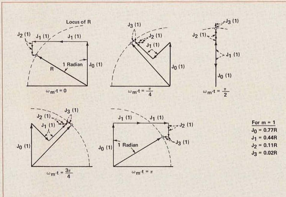
Figure I-6. Phasor diagrams of an FM signal with a modulation index m = 1 . Different diagrams corresponding to different points in the cycle of the sinusoidal modulating wave.
