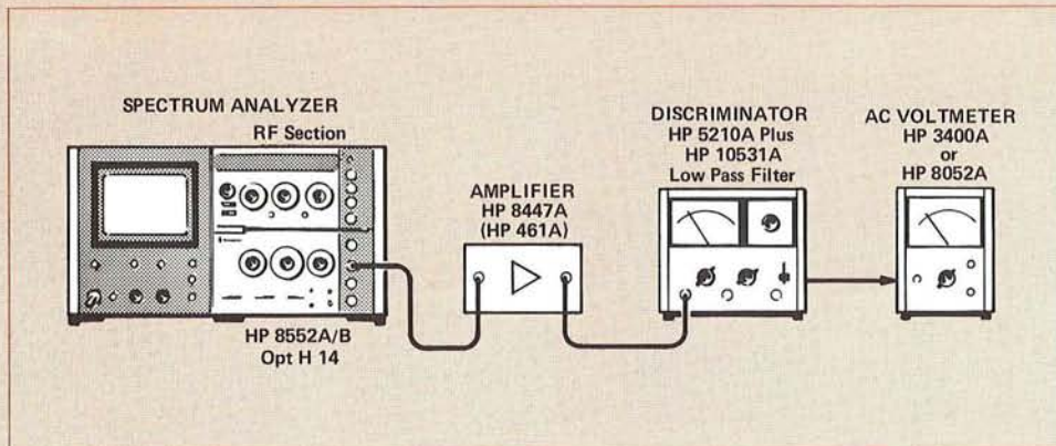
Figure 20. A typical setup.
