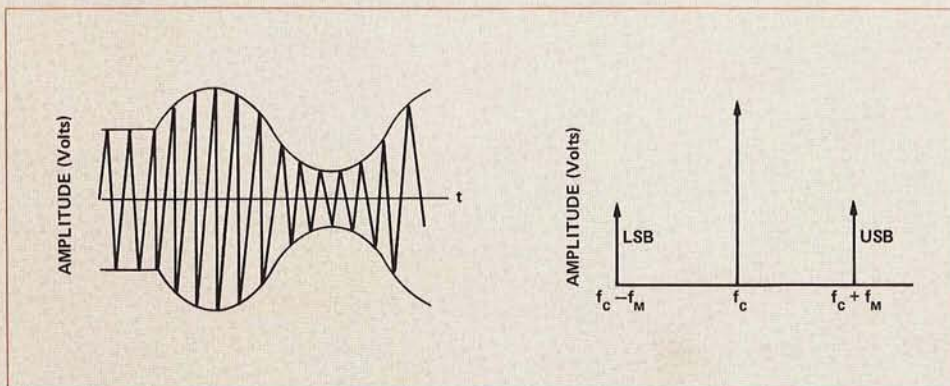
Figure 1A. Time domain (oscilloscope) display of an amplitude modulated carrier.
