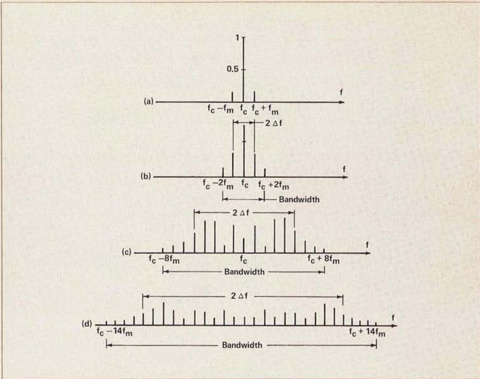
Figure 12. Amplitude-frequency spectrum, FM signal (sinusoidal modulating signal, f_m fixed, amplitude varying). (a) m = 0.2 ; (b) m = 1 ; (c) m = 5 ; (d) m = 10 .
