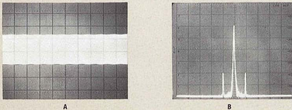
Figure 3. Time and frequency domain views of low level (2%) AM.
